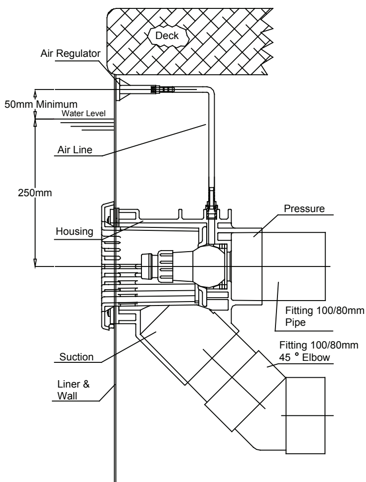
Fig 5. BADU®STREAM II in Fibreglass Pool
